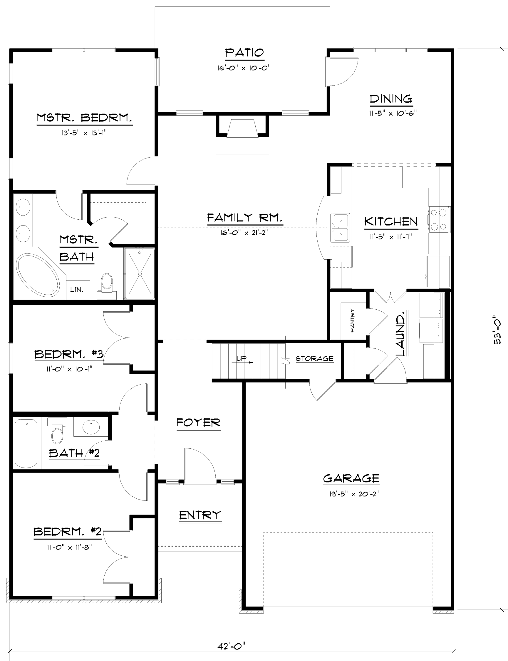
MAIN LEVEL FLOOR PLAN
